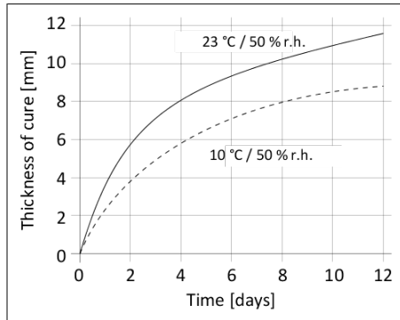
Diagram 1: Curing speed of Sikaflex® Fix
