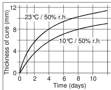
Diagram 1: Curing speed for Sikaflex®-221
