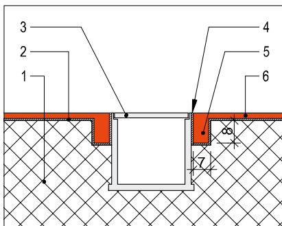
Connection to drainage channels and gullies
