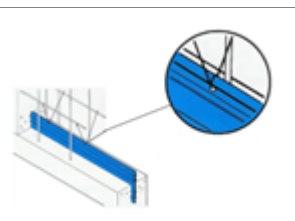
Heat Welding of Waterstops
