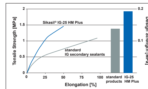
Comparison of stress-strain curve and design strength of Sikasil® IG-25 HM Plus with standard IG products
