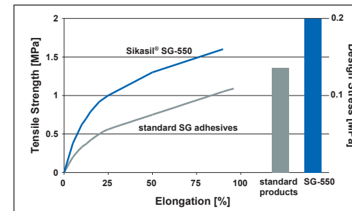
Comparison of stress-strain curve and design strength of Sikasil® SG-550 with standard SG adhesives
