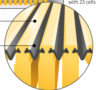
Side view Sika modular flexible joint with 23 cells
