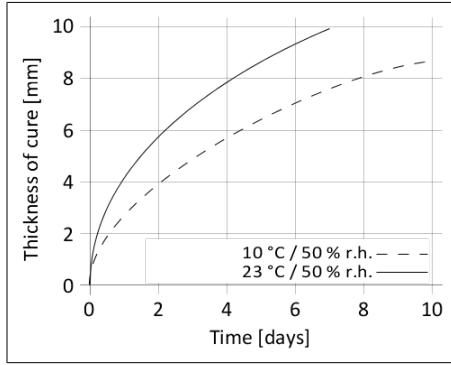
Diagram 1: Curing speed SikaTack® Go P2G
