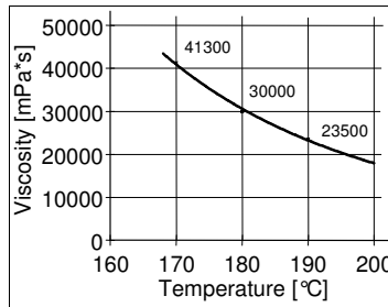
Diagram 1: Viscosity of SikaMelt®-9170 as a function of temperature
