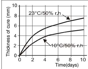
Diagram 1: Curing speed for Sikaflex®-521 UV
