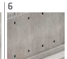
6 SikaSwell® Rings and Plugs Sikadur® 31 Sealing tie bar holes
