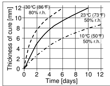
Diagram 1: Curing speed for Sikaflex®-252
